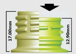
PCO 1881 | PCO 26/22
