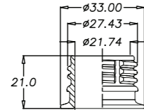
28mm PCO 1810
