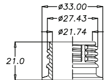
28mm PCO 1810
